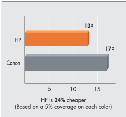
CPP Graph (US cents)
