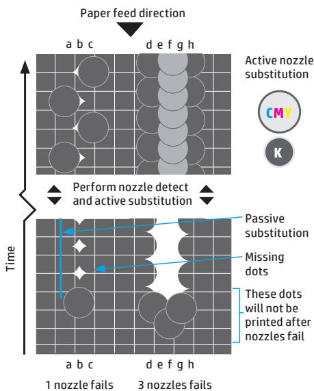
Figure 7: Nozzle substitution
