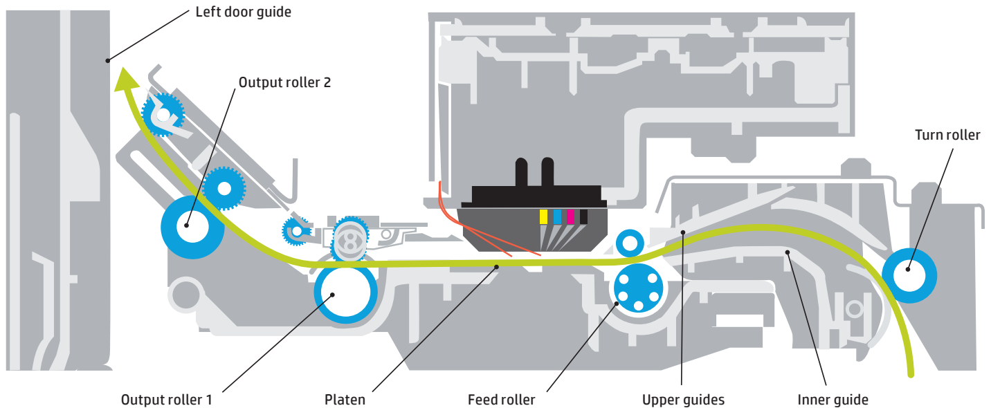
Figure 9: Cross-section of paper transport system
