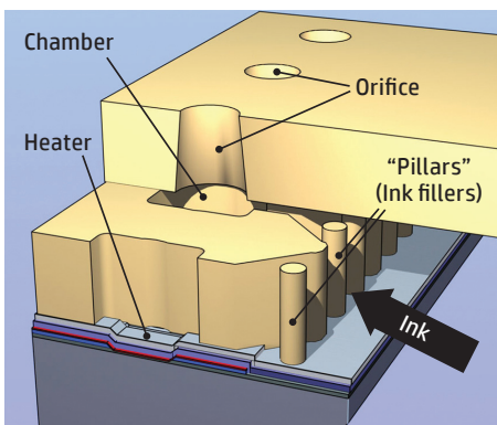
Figure 2: Cutaway view of an SPT-based drop generator
