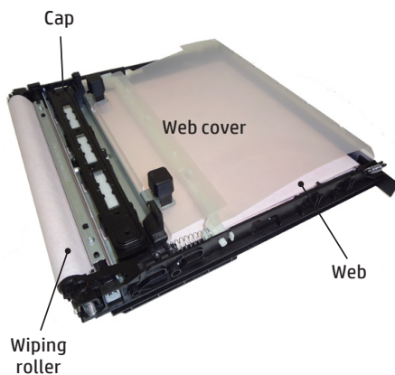
Figure 8: Printhead service station cassette
