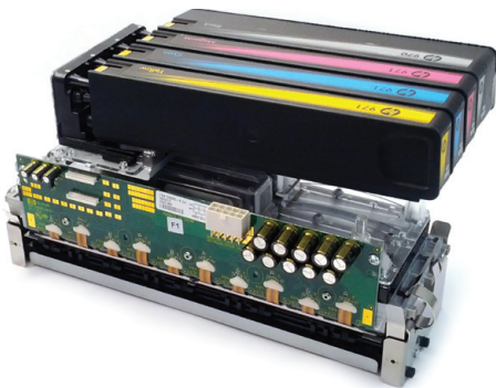
Figure 3: Page-wide writing engine assembly
